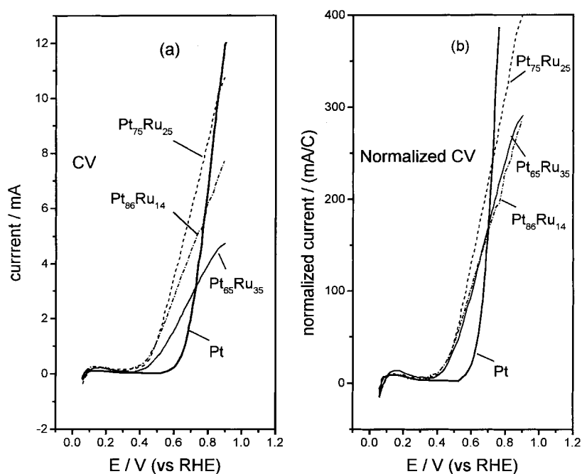
Fig. 2. Cyclic voltammograms of methanol oxidation at different PtRu electrodeposits on sputtered gold, 0.1 \text{ M CH}_3\text{OH} in 0.1 \text{ M HClO}_4 , 10 \text{ mV s}^{-1} , geometric surface 1.13 \text{ cm}^2 , (a) without normalization, (b) normalized as described in paragraph 2.5 (Figure 1(a)), dividing the current by the corresponding Q_{ox} value (Table 1).
