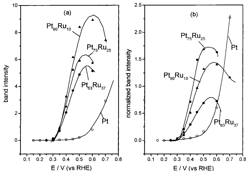
Fig. 4. Potential step voltammograms of integrated FTIR band intensities of CO 2 ( \nu = 2341 \text{ cm}^{-1} ) during methanol oxidation at different PtRu electrodeposits on a smooth gold surface. 0.1 M CH 3 OH + 0.1 M HClO 4 , 256 scans, 8 cm -1 resolution. (a) Without normalization, (b) with normalization according to paragraph 2.5 (Figure 1(c)).
